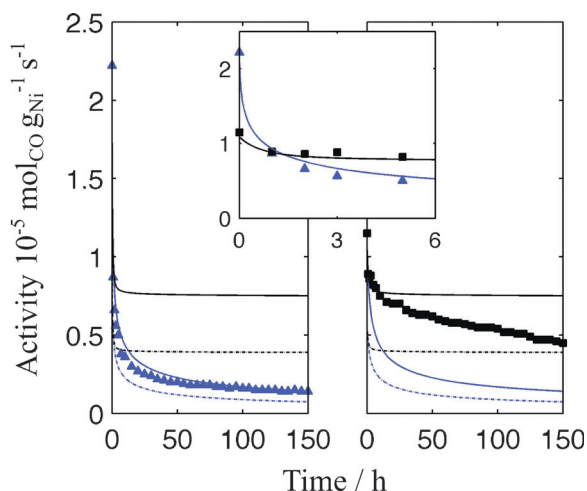
Figure 3. Modelling the deactivation of catalysts Ni-C3 (left) and Ni-D8 (right). The symbols represent the experimental data, the lines the model predictions: unhindered particle growth (blue) and confined growth (black). The solid and dashed lines are obtained using the TOF of the fresh and spent catalysts, respectively, which accounts for carbon buildup. The initial particle size distribution played a large role only in the first hour of the modelling predictions (Figure S11). In the inset, the unhindered growth model is used for Ni-C3 and the confined model for Ni-D8.
